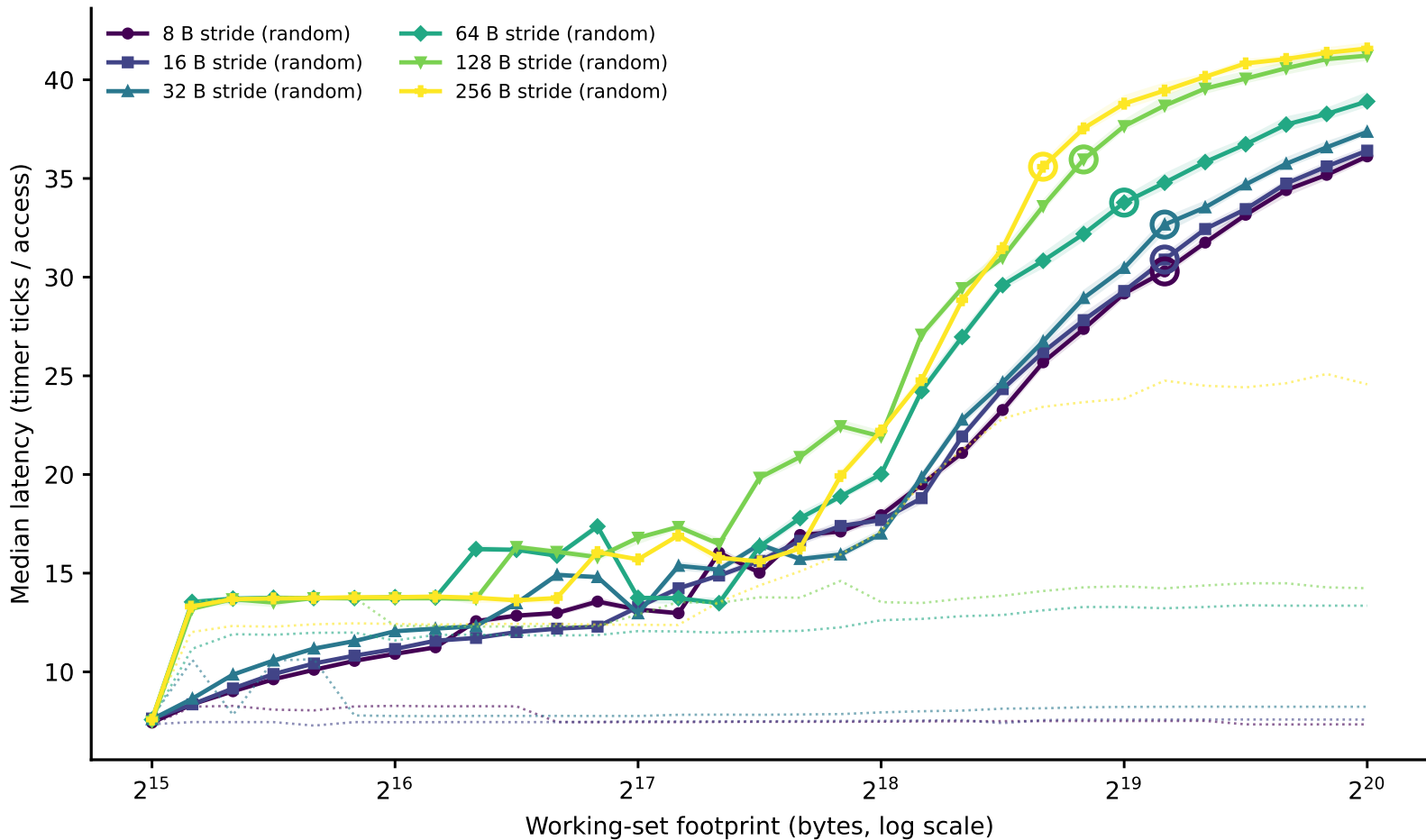
ookay: line-size family of curves (dependent pointer chase) (Phase I timing-only, level boundary=262144B window=[32768,1048576])
