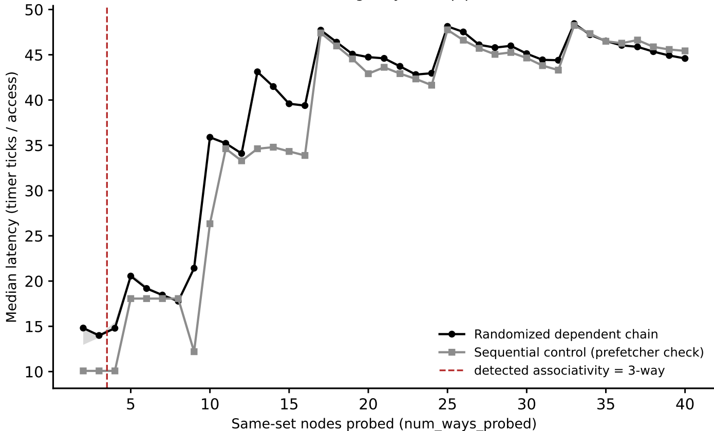
sunbird: associativity sweep, L2 (stride=256 KiB) (Phase I timing-only, auto pipeline)
