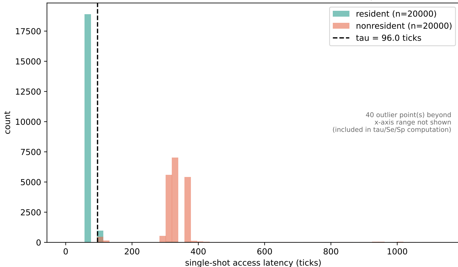
Calibration distributions: resident vs. nonresident (skylark)
