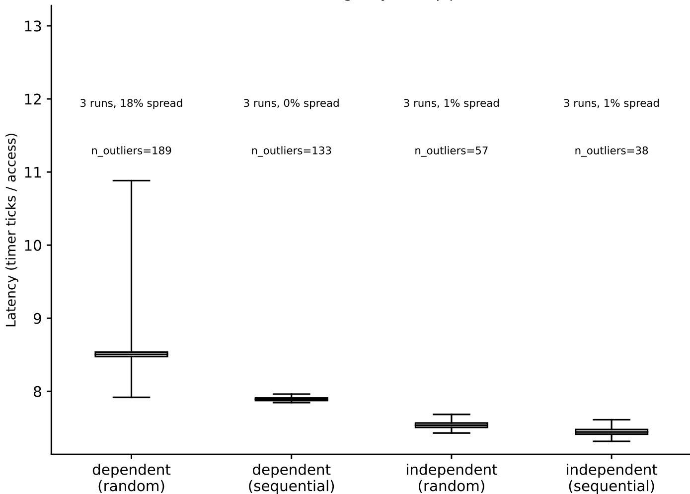
charnwood: hit-latency box plots, L1 (footprint=32 KiB) (Phase I timing-only, auto pipeline)
