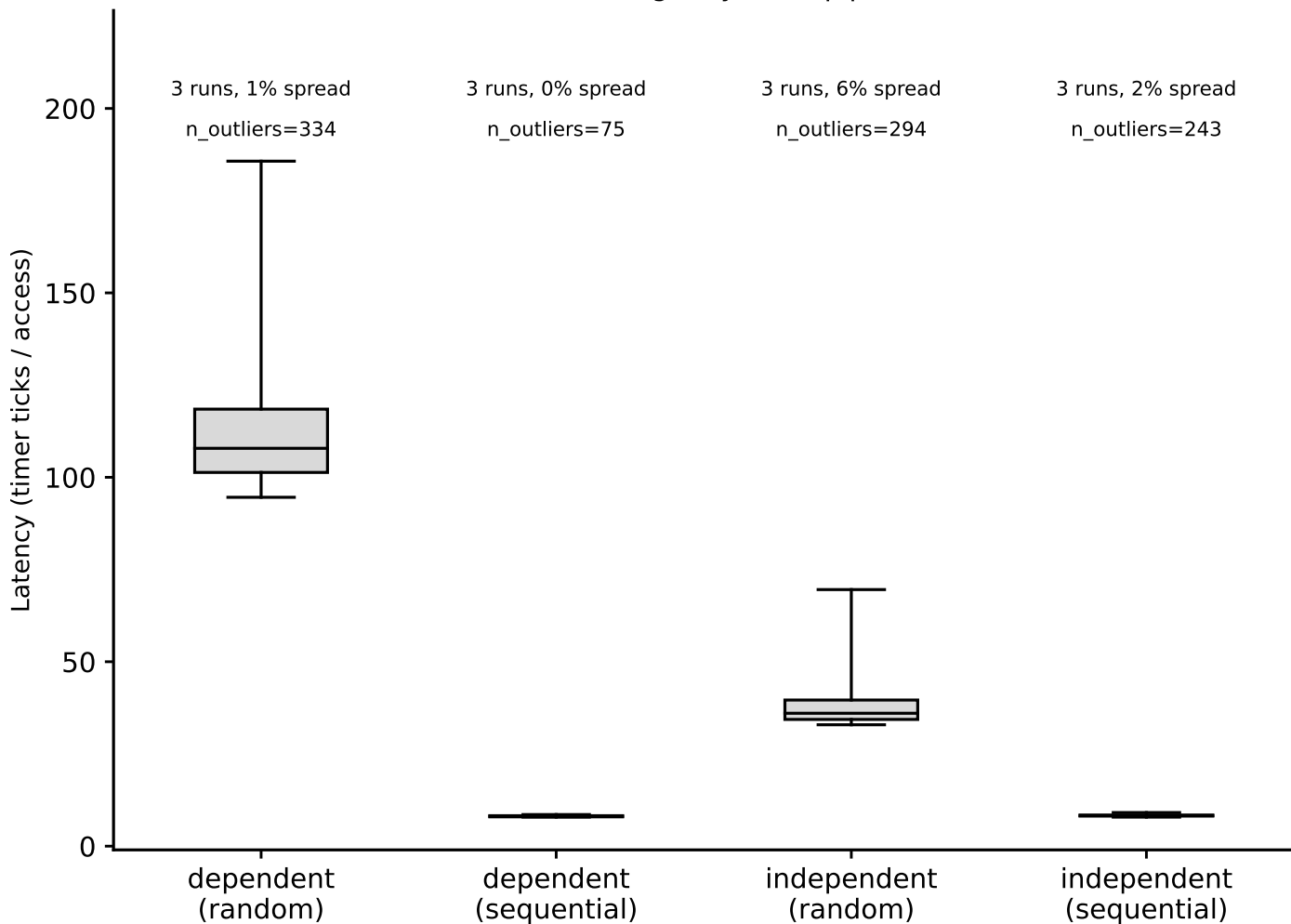
charnwood: hit-latency box plots, LLC (footprint=8 MiB) (Phase I timing-only, auto pipeline)
