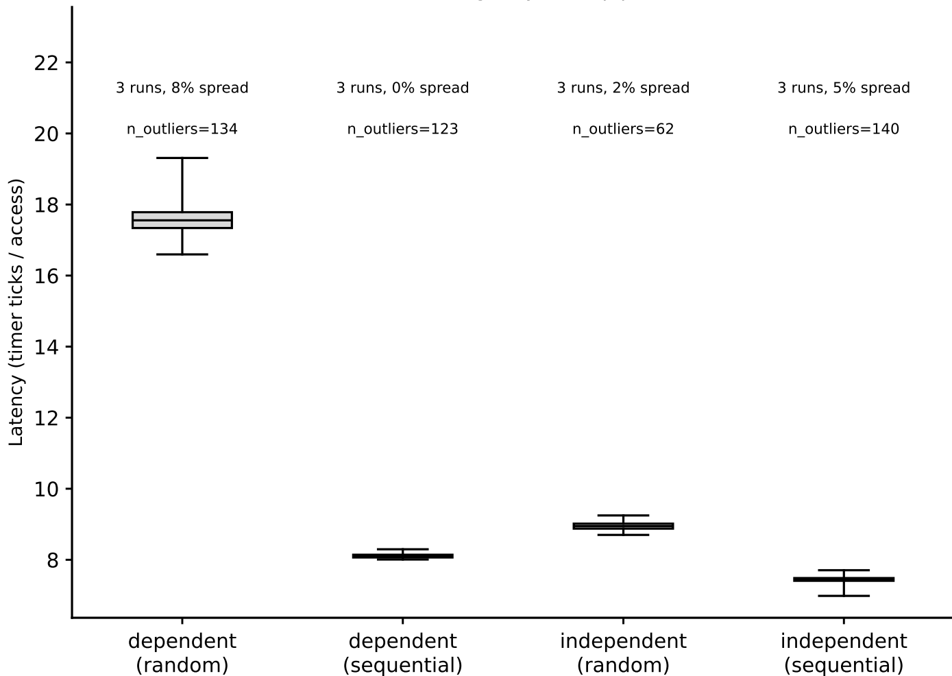
ookay: hit-latency box plots, L2 (footprint=256 KiB) (Phase I timing-only, auto pipeline)
