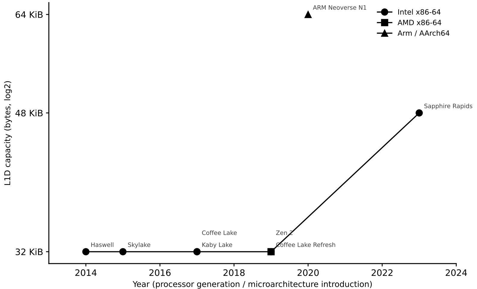
L1D capacity vs. year
