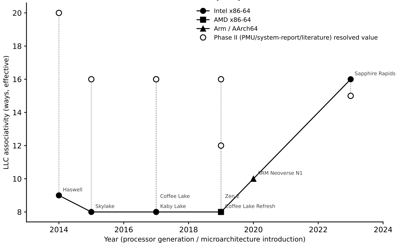
LLC associativity vs. year
