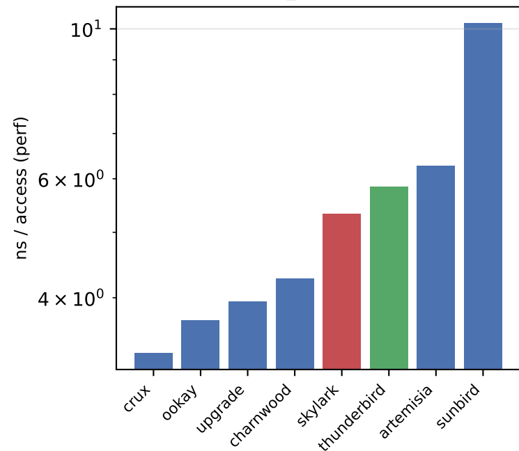
L1_resident
