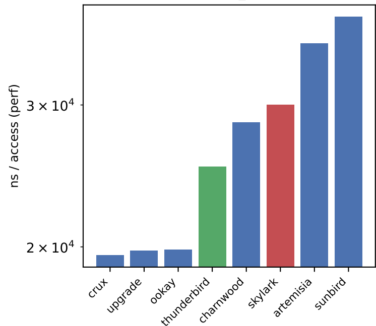
beyond_LLC
