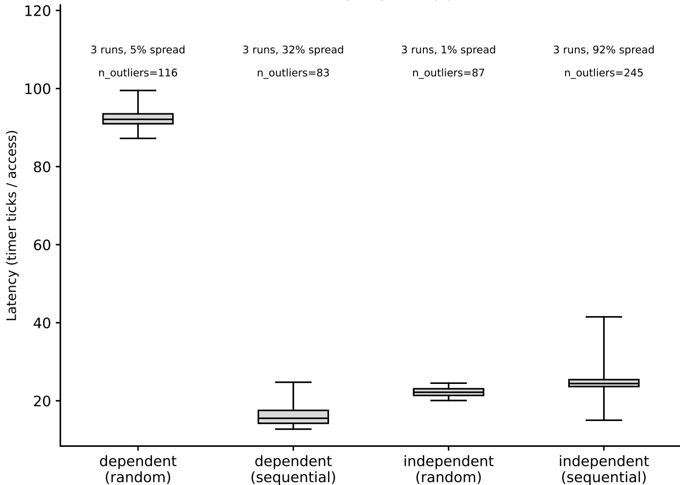
artemisia: hit-latency box plots, LLC (footprint=30 MiB) (Phase I timing-only, auto pipeline)
