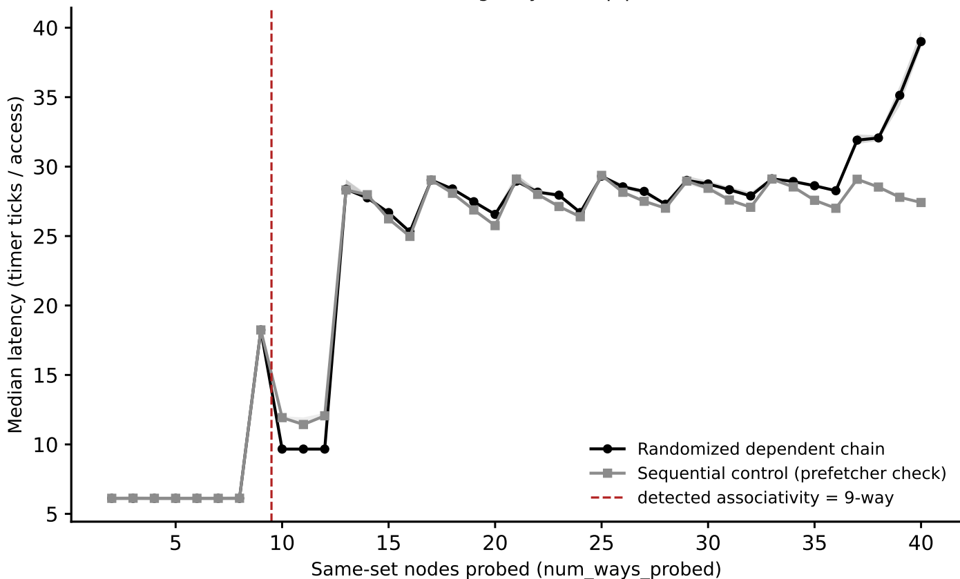
skylark: associativity sweep, L2 (stride=512 KiB) (Phase I timing-only, auto pipeline)
