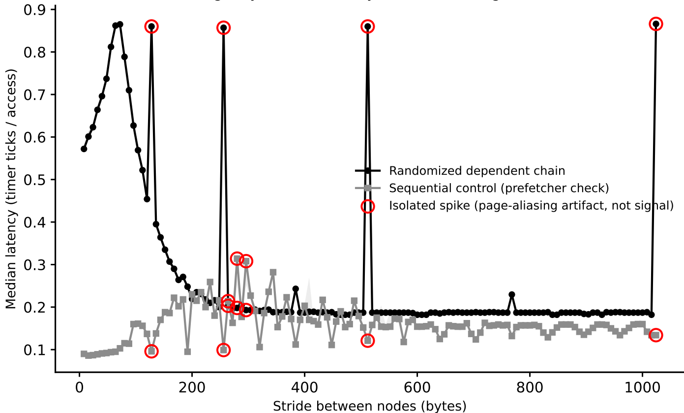
thunderbird: line-size sweep (dependent pointer chase), footprint=2 MiB (Phase I timing-only, level boundary=1048576B, single-curve method)
