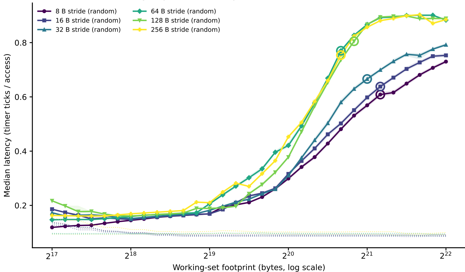
thunderbird: line-size family of curves (dependent pointer chase) (Phase I timing-only, level boundary=1048576B window=[131072,4194304])
