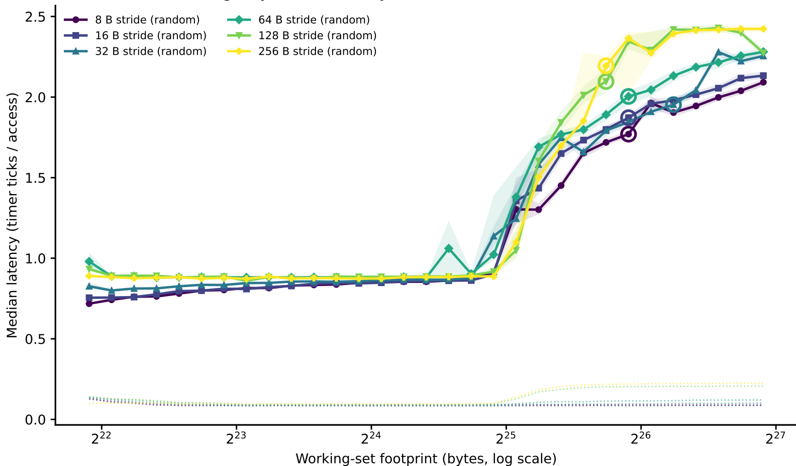
thunderbird: line-size family of curves (dependent pointer chase) (Phase I timing-only, level boundary=31457280B window=[3932160,125829120])
