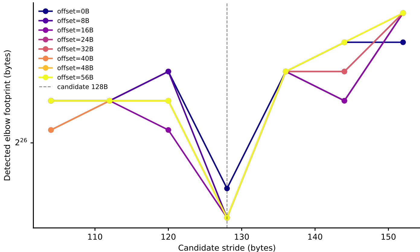
thunderbird: line-size elbow vs. stride, by node-0 offset (Phase I timing-only, level boundary=31457280B, step-4 alignment refinement)
