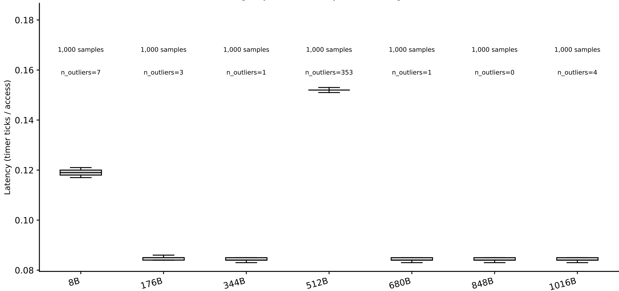
thunderbird: line-size box plots, random pattern (whiskers = p5/p95) (Phase I timing-only, level boundary=65536B, single-curve method)
