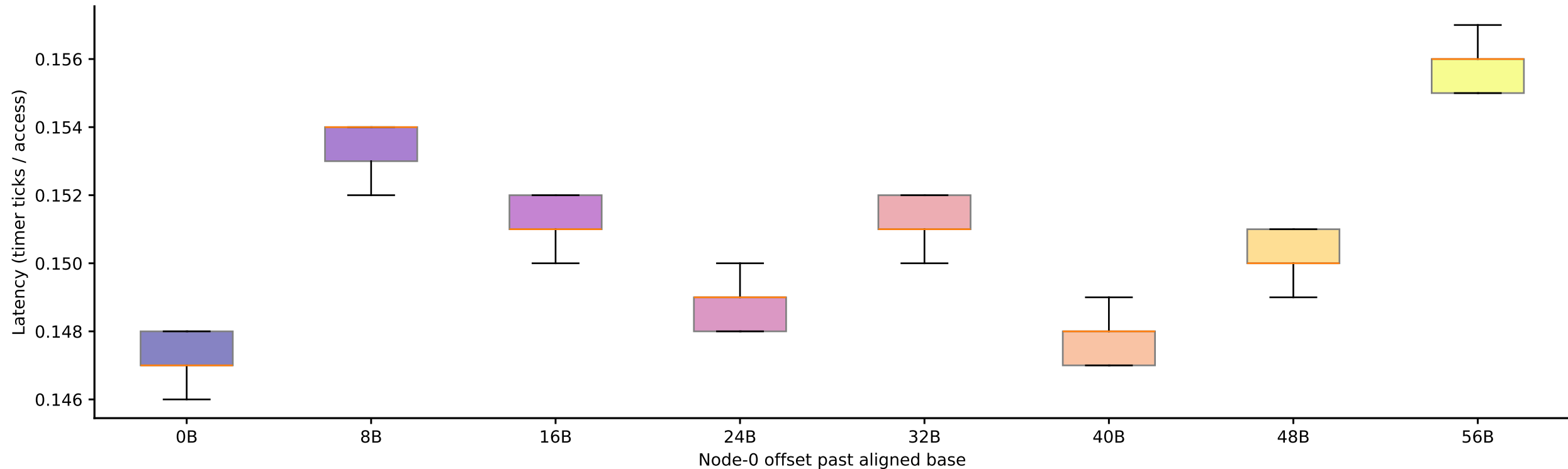
thunderbird: candidate stride 64 B at footprint 80.625 KiB, by offset (Phase I timing-only, level boundary=65536B, step-4 alignment refinement)
