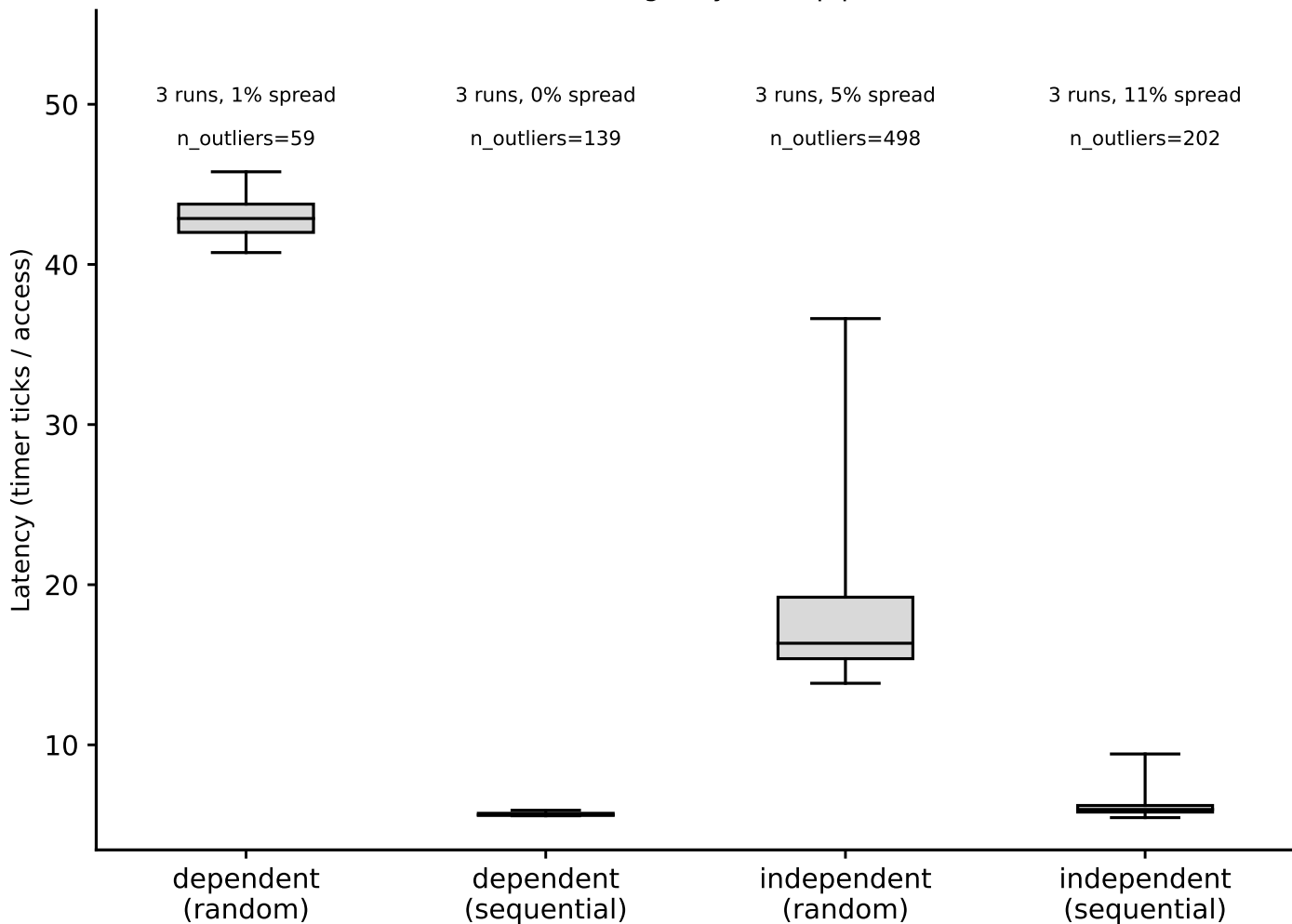
crux: hit-latency box plots, LLC (footprint=8 MiB) (Phase I timing-only, auto pipeline)
