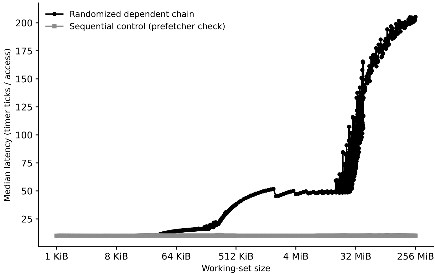
sunbird: capacity sweep (dependent pointer chase)
