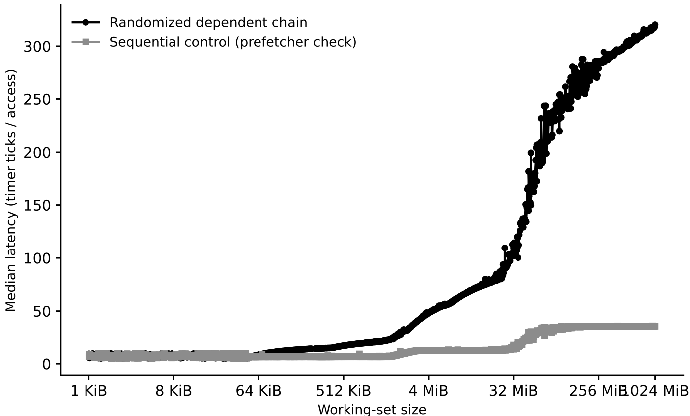
artemisia: capacity sweep (dependent pointer chase) (Phase I timing-only, auto pipeline + manual tail/mid extension repeats, core 20)
