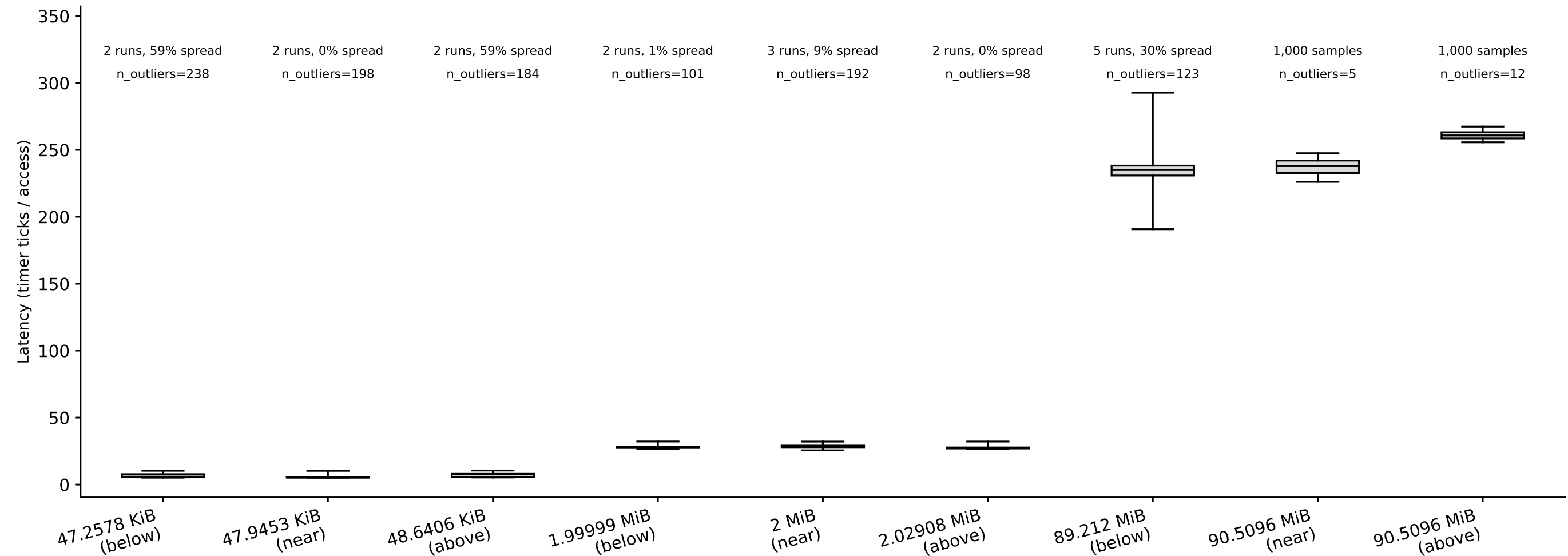
artemisia: capacity box plots, random pattern (whiskers = p5/p95) tested boundaries: 48 KiB, 2 MiB, 90 MiB
