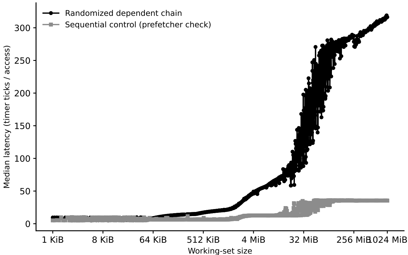
artemisia: capacity sweep (dependent pointer chase)
