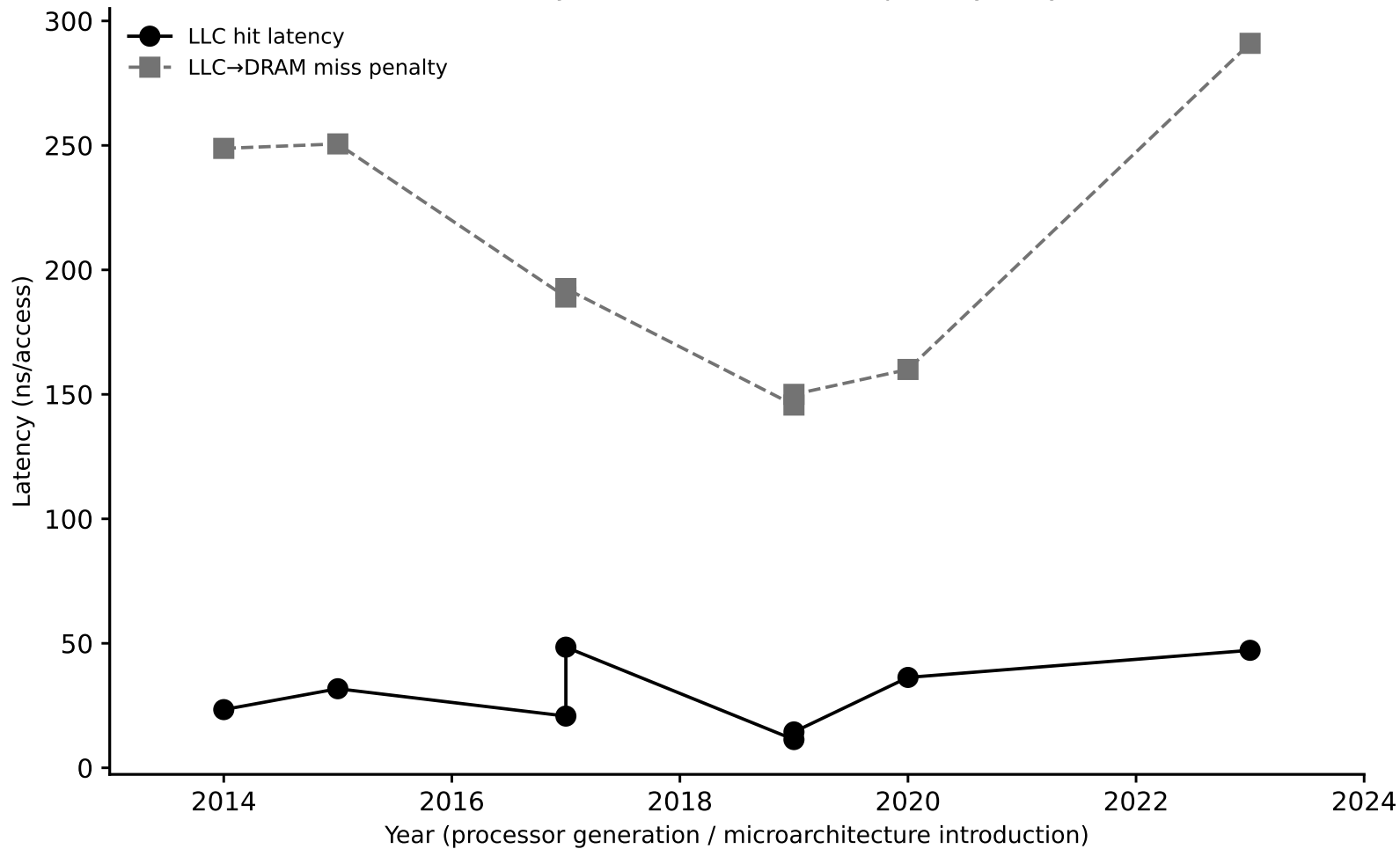
LLC hit latency and LLC→DRAM miss penalty vs. year
