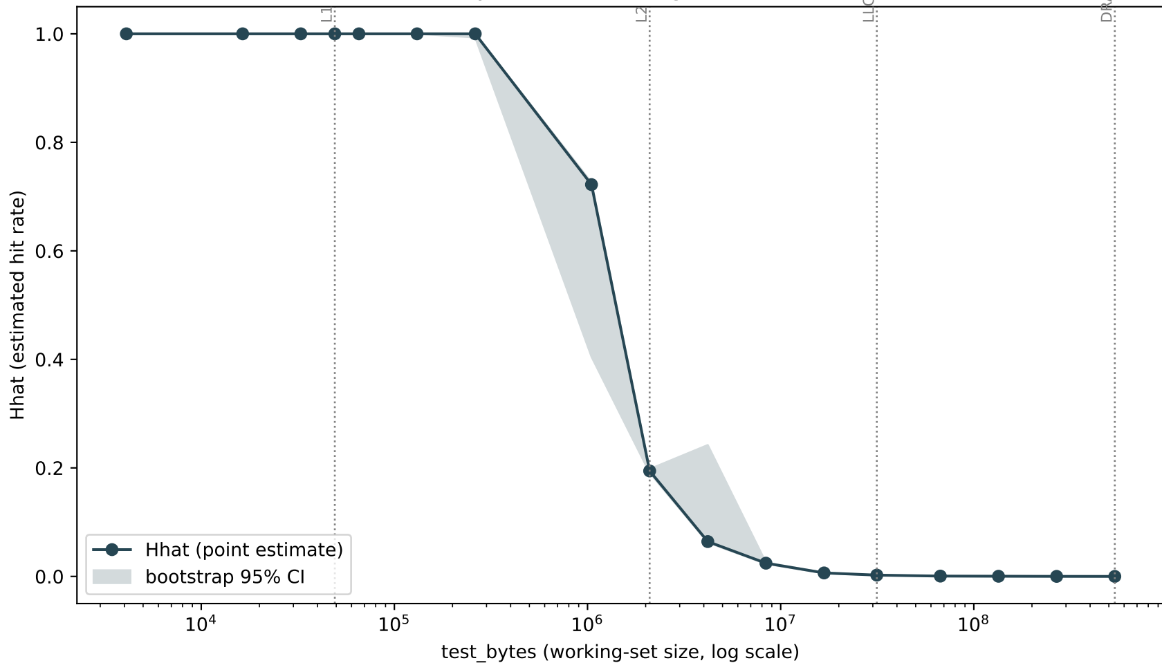
Software-only Hhat vs. working-set size (artemisia)
