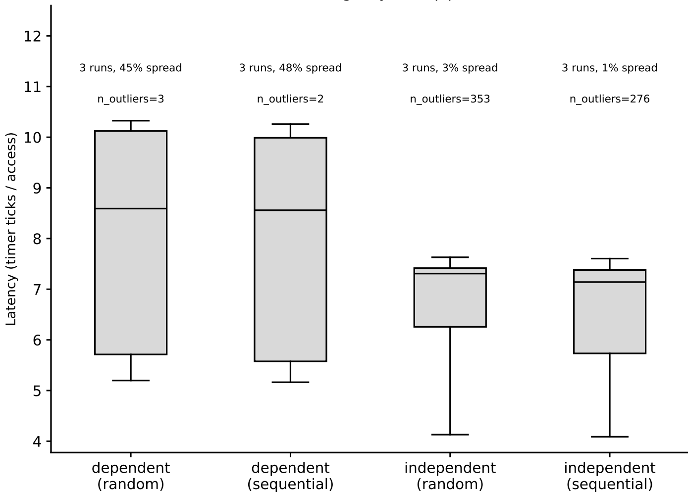
artemisia: hit-latency box plots, L1 (footprint=48 KiB) (Phase I timing-only, auto pipeline)
