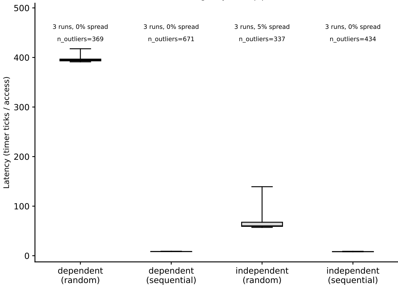
charnwood: hit-latency box plots, DRAM (footprint=512 MiB) (Phase I timing-only, auto pipeline)
