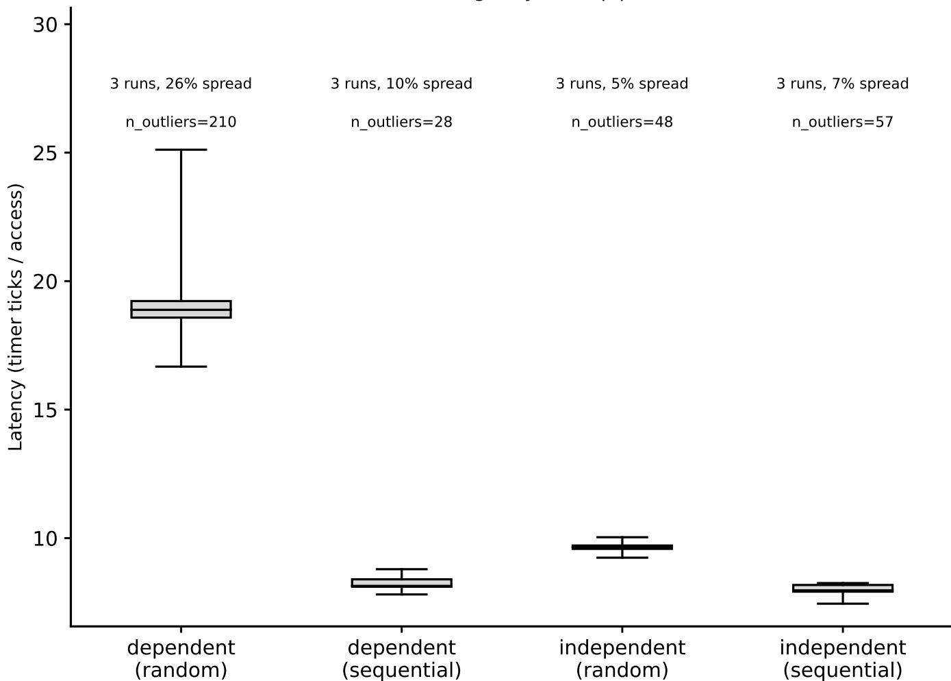
charnwood: hit-latency box plots, L2 (footprint=256 KiB) (Phase I timing-only, auto pipeline)
