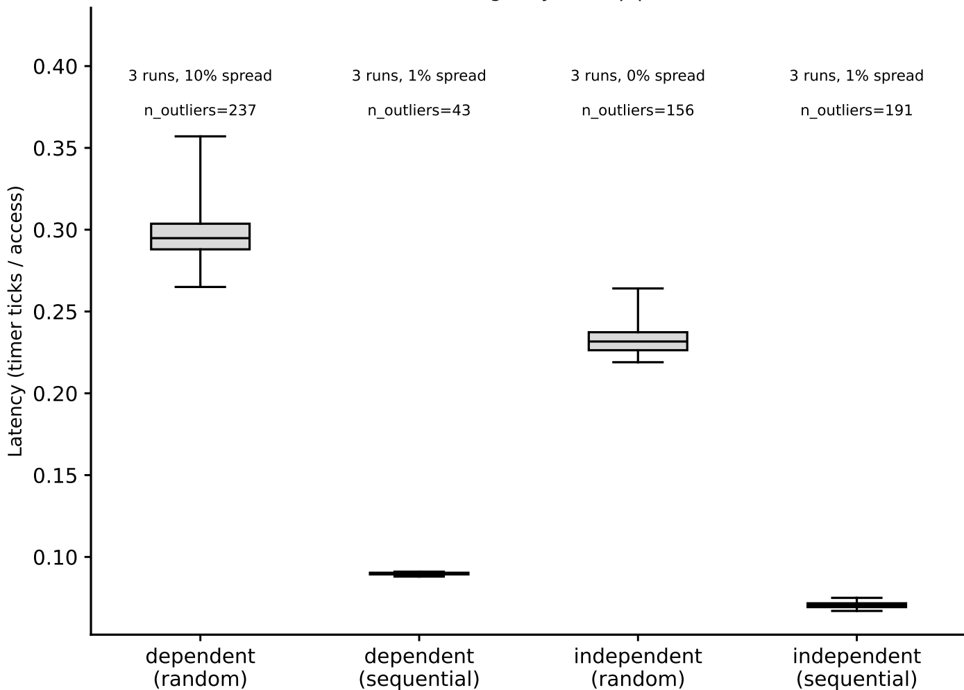
thunderbird: hit-latency box plots, L2 (footprint=1 MiB) (Phase I timing-only, auto pipeline)
