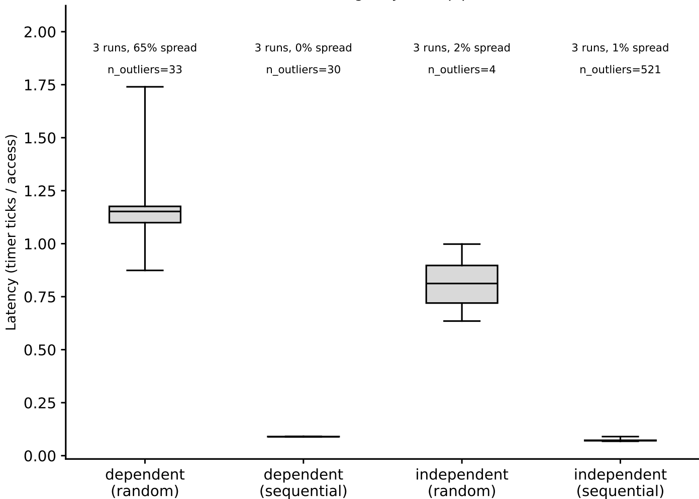
thunderbird: hit-latency box plots, LLC (footprint=30 MiB) (Phase I timing-only, auto pipeline)
