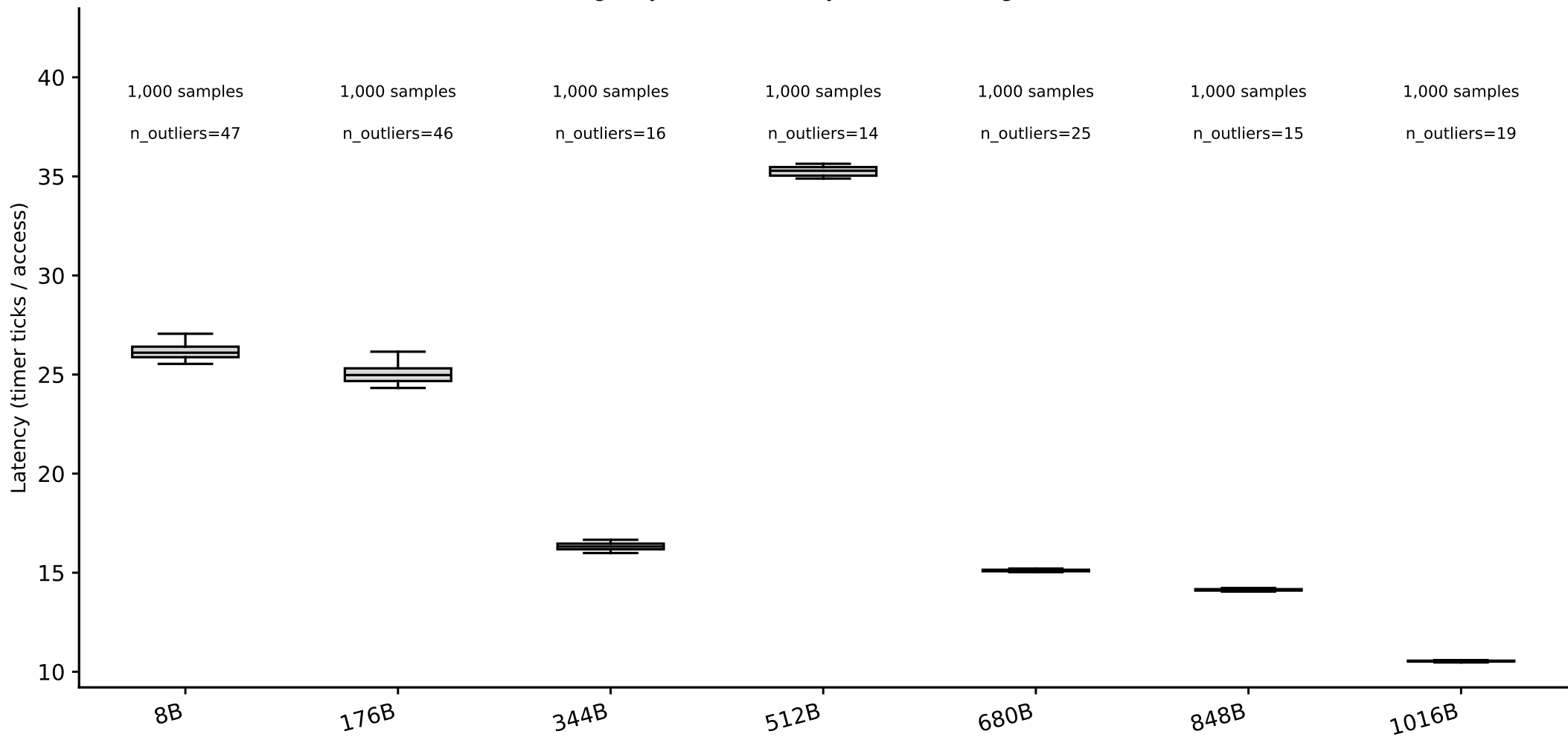
upgrade: line-size box plots, random pattern (whiskers = p5/p95) (Phase I timing-only, level boundary=262144B, single-curve method)
