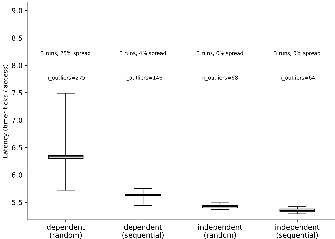
crux: hit-latency box plots, L1 (footprint=32 KiB) (Phase I timing-only, auto pipeline)
