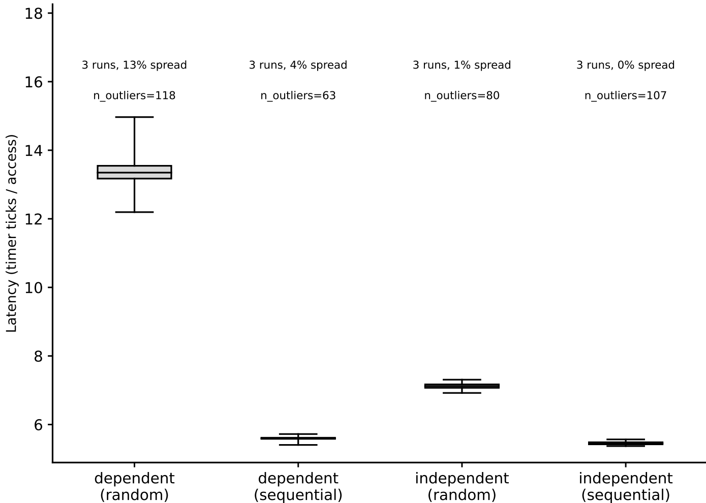
crux: hit-latency box plots, L2 (footprint=256 KiB) (Phase I timing-only, auto pipeline)
