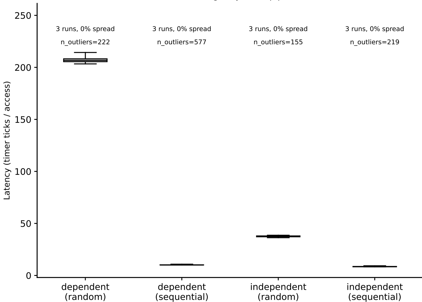
sunbird: hit-latency box plots, DRAM (footprint=512 MiB) (Phase I timing-only, auto pipeline)
