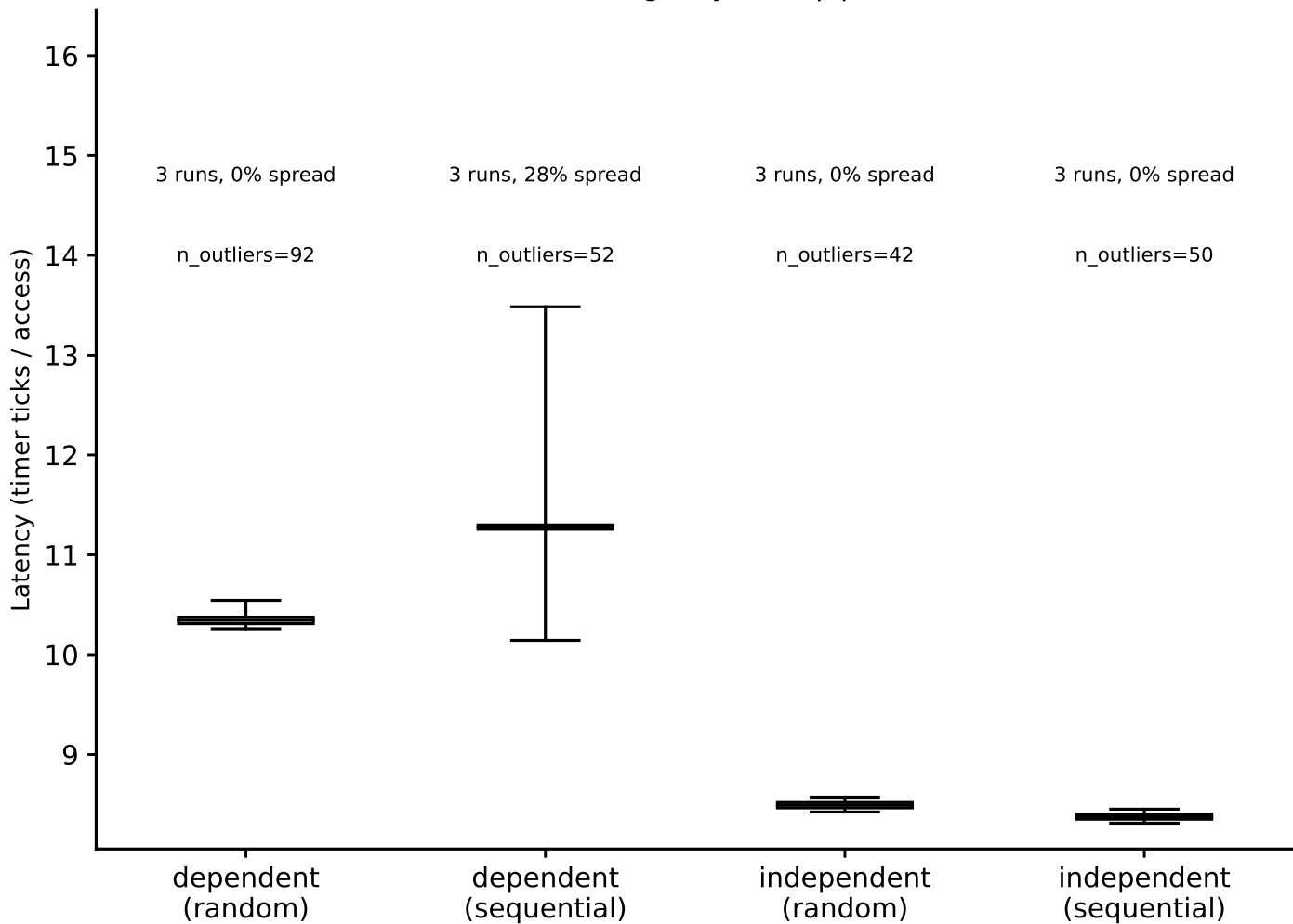
sunbird: hit-latency box plots, L1 (footprint=32 KiB) (Phase I timing-only, auto pipeline)
