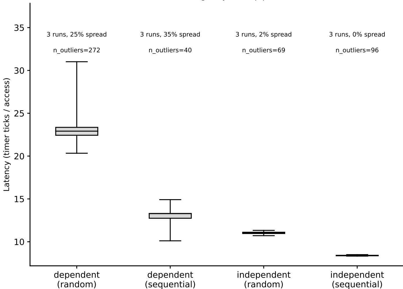
sunbird: hit-latency box plots, L2 (footprint=256 KiB) (Phase I timing-only, auto pipeline)
