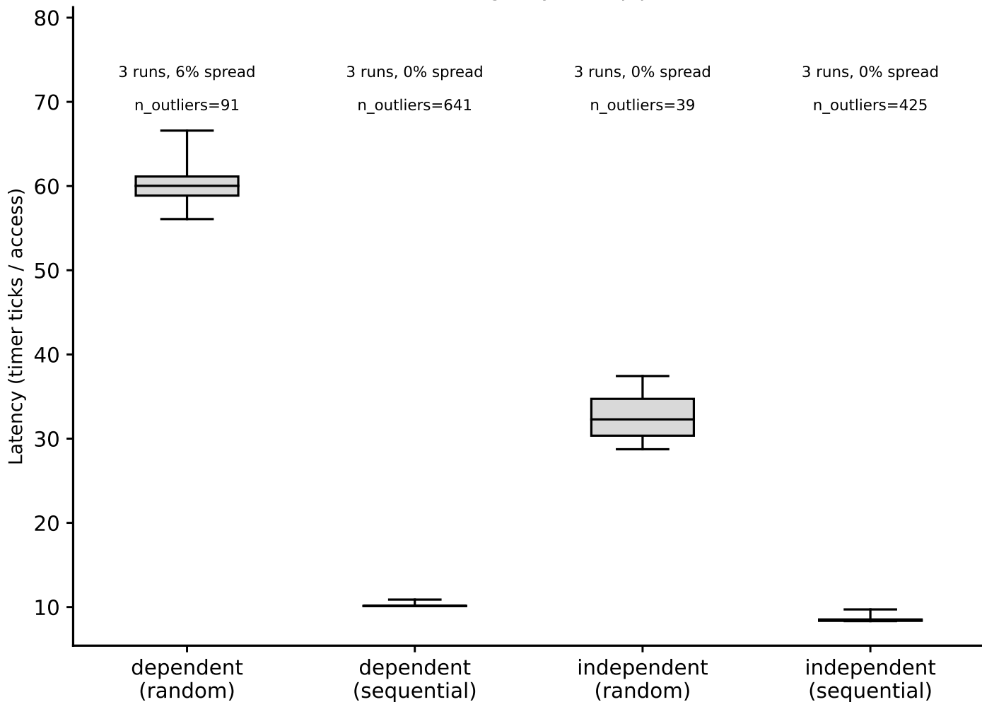
sunbird: hit-latency box plots, LLC (footprint=30 MiB) (Phase I timing-only, auto pipeline)
