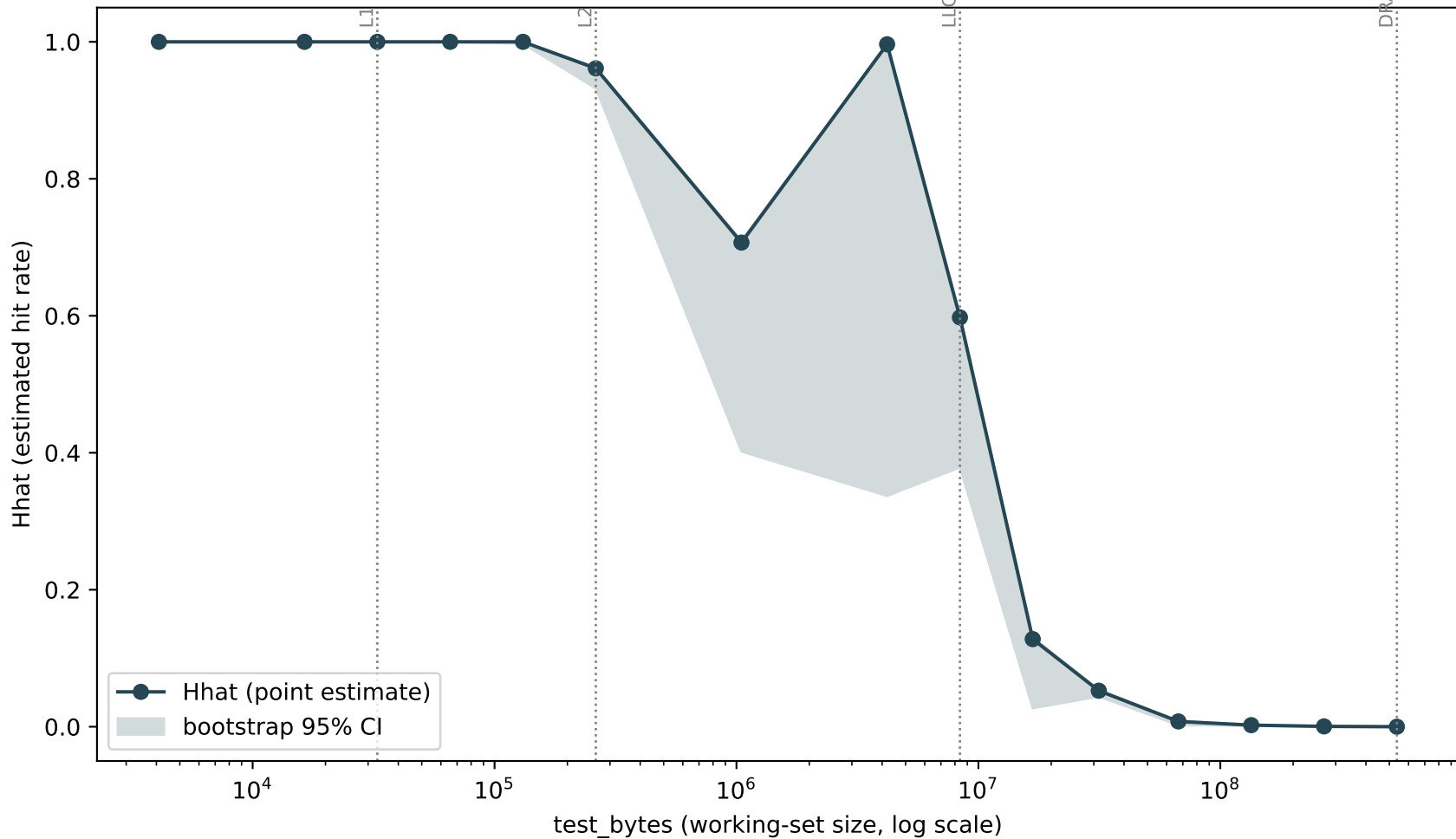
Software-only Hhat vs. working-set size (ookay)
