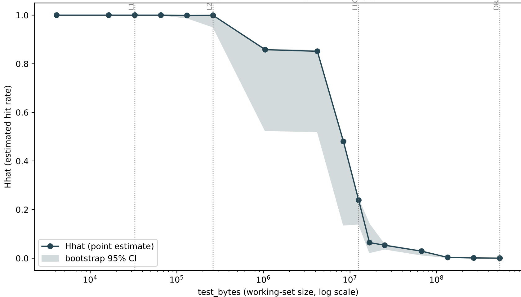
Software-only Hhat vs. working-set size (upgrade)
