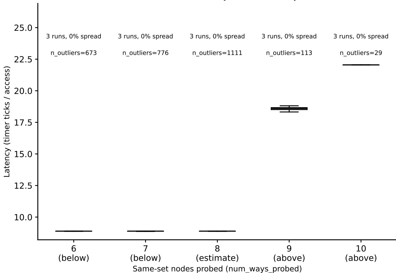
hazel_broadwell/phase1_v2: associativity box plots, L1, random pattern (whiskers = p5/p95) (Phase I timing-only, auto pipeline) detected associativity estimate: 8-way
