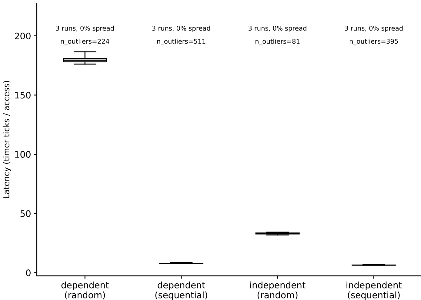
hazel_broadwell/phase1_v2: hit-latency box plots, DRAM (footprint=512 MiB) (Phase I timing-only, auto pipeline)
