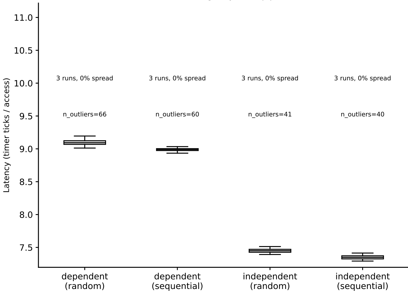
hazel_broadwell/phase1_v2: hit-latency box plots, L1 (footprint=32 KiB) (Phase I timing-only, auto pipeline)
