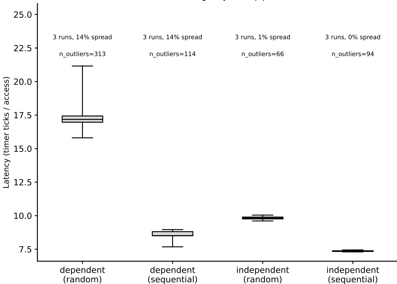
hazel_broadwell/phase1_v2: hit-latency box plots, L2 (footprint=256 KiB) (Phase I timing-only, auto pipeline)
