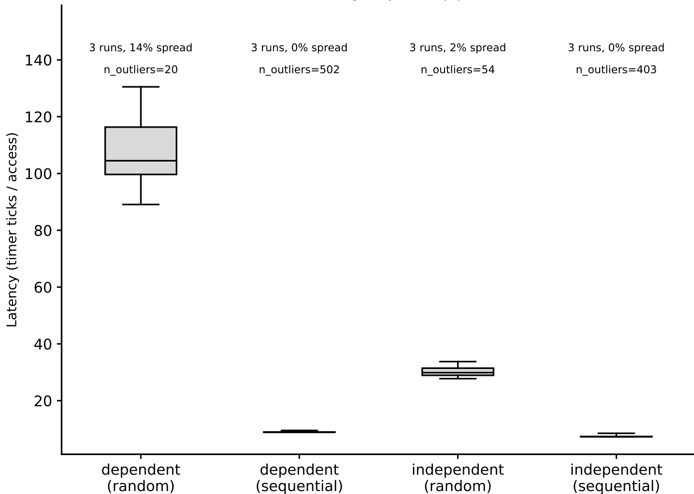
hazel_broadwell/phase1_v2: hit-latency box plots, LLC (footprint=32 MiB) (Phase I timing-only, auto pipeline)
