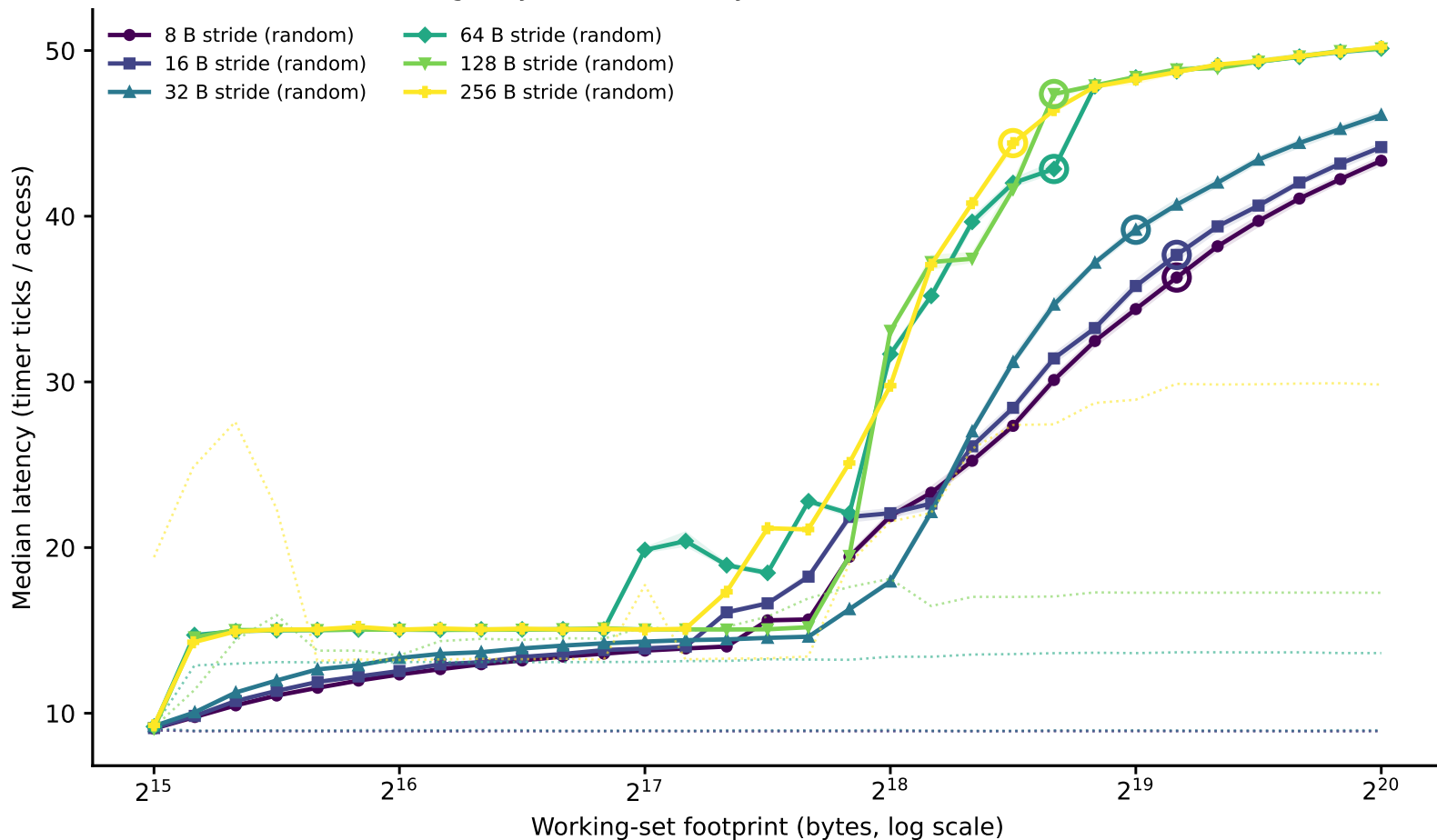
hazel_broadwell/phase1_v2: line-size family of curves (dependent pointer chase) (Phase I timing-only, level boundary=262144B window=[32768,1048576])
