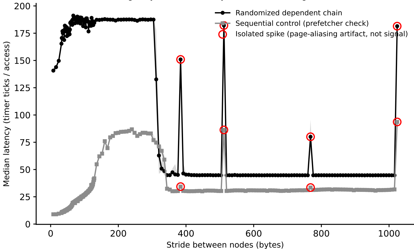
hazel_broadwell/phase1_v2: line-size sweep (dependent pointer chase), footprint=64 MiB (Phase I timing-only, level boundary=33554432B, single-curve method)
