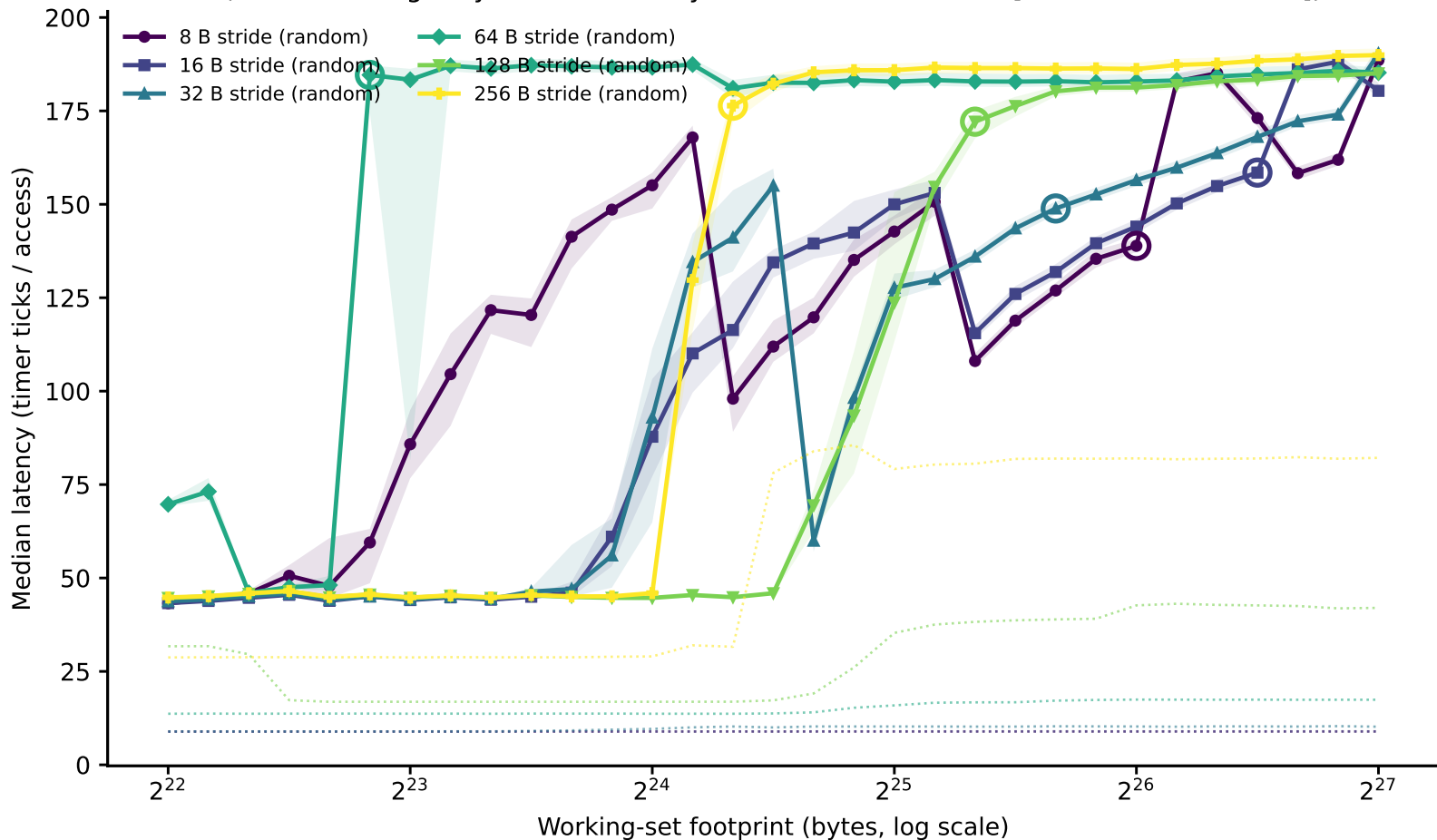
hazel_broadwell/phase1_v2: line-size family of curves (dependent pointer chase) (Phase I timing-only, level boundary=33554432B window=[4194304,134217728])
