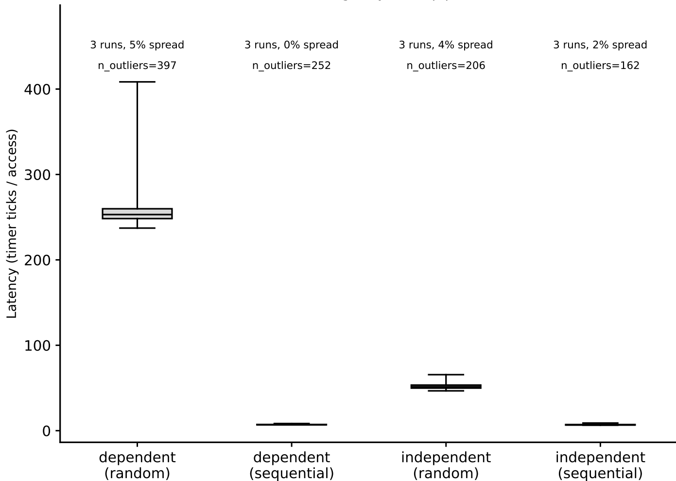
hazel_cascadelake/phase1_v2: hit-latency box plots, DRAM (footprint=512 MiB) (Phase I timing-only, auto pipeline)
