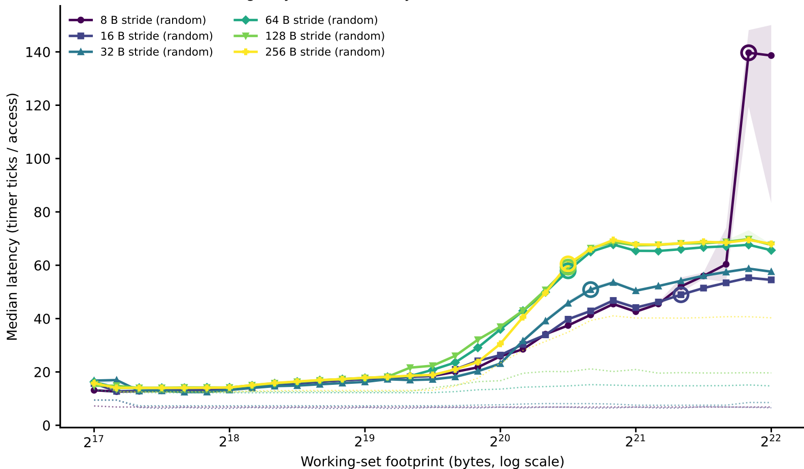
hazel_cascadelake/phase1_v2: line-size family of curves (dependent pointer chase) (Phase I timing-only, level boundary=1048576B window=[131072,4194304])
