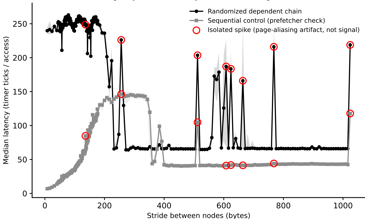
hazel_cascadelake/phase1_v2: line-size sweep (dependent pointer chase), footprint=32 MiB (Phase I timing-only, level boundary=16777216B, single-curve method)
