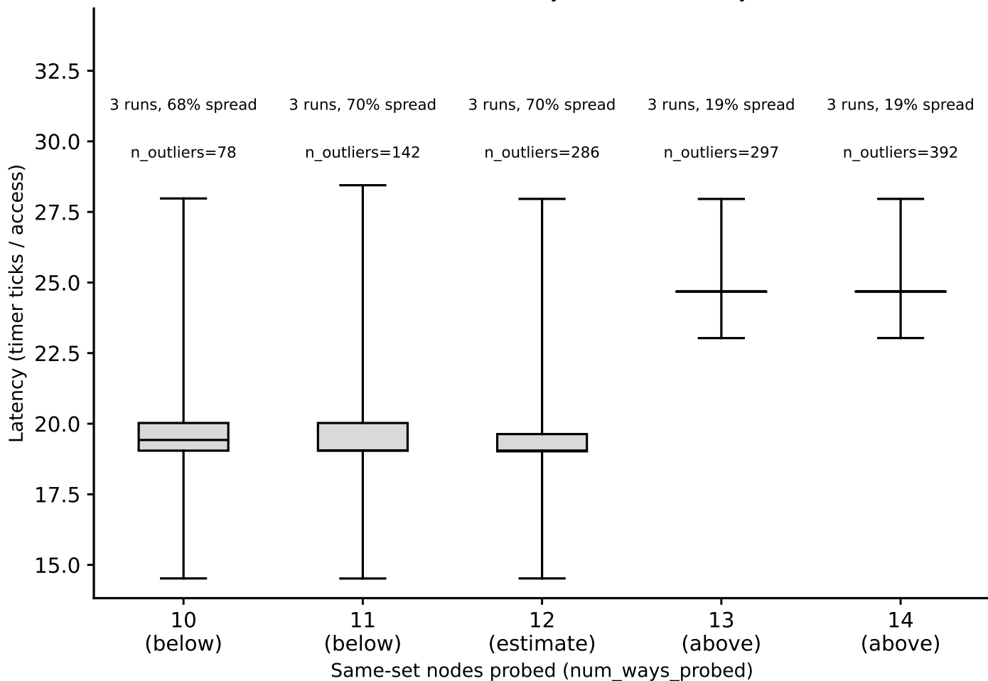
hazel_icelake_6326/phase1_v2: associativity box plots, L1, random pattern (whiskers = p5/p95) (Phase I timing-only, auto pipeline) detected associativity estimate: 12-way
